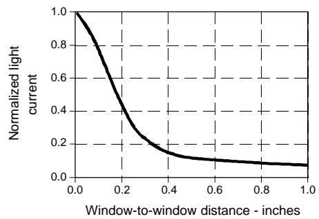
Fig. 6 Coupling Characteristics SE3450 with SD3443
